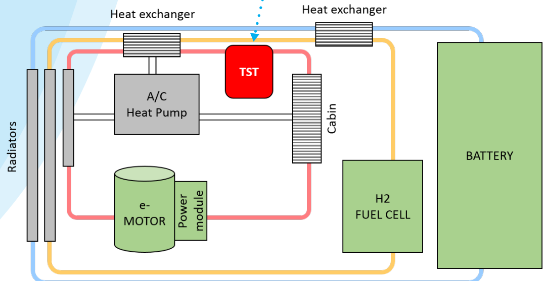
Vehicle Thermal Management System
